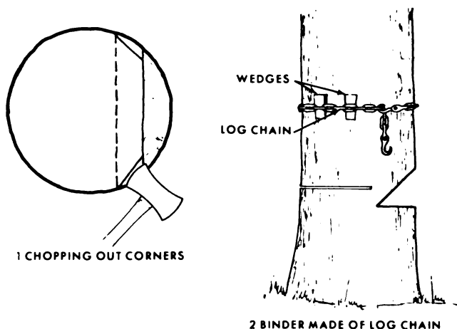
Figure 5-12. Methods used to prevent splitting a tree.
